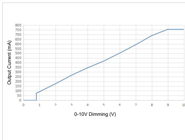
Dimming Curve
